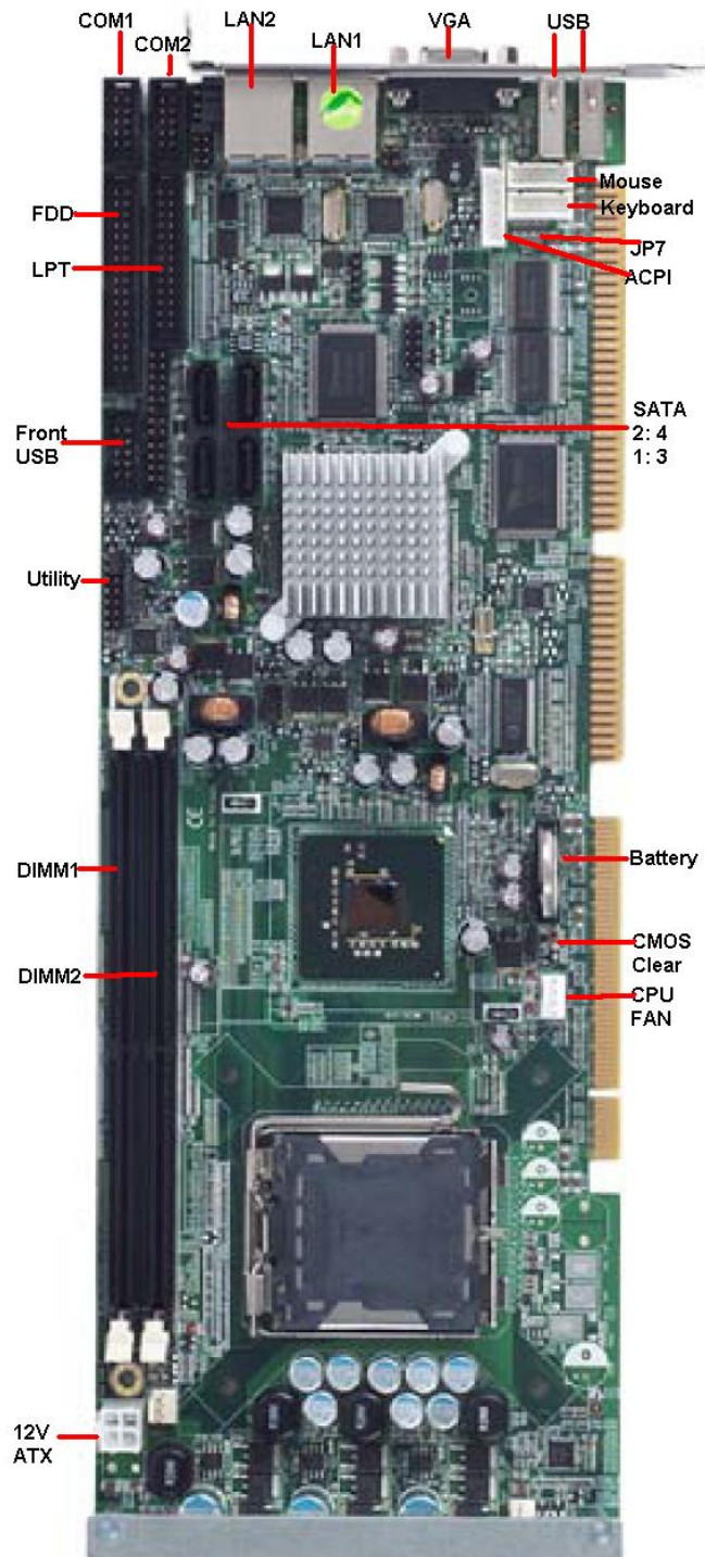
Figure 1: Connector Locations
