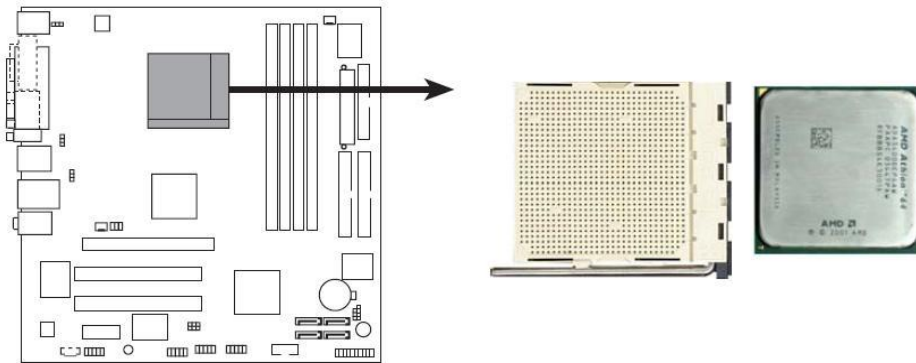
Figure 5: CPU Installation
