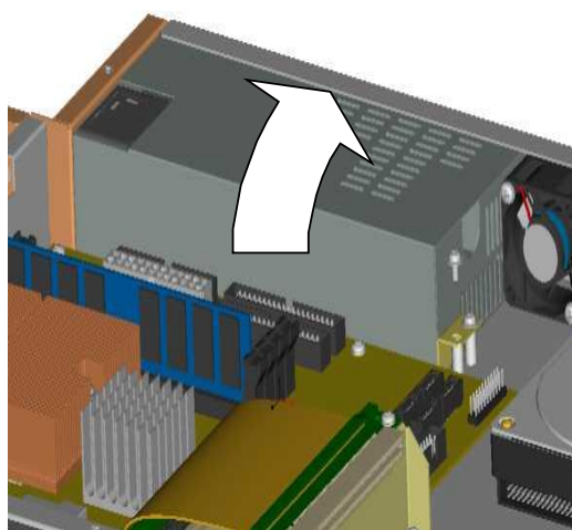
Figure 16: PSU removal
