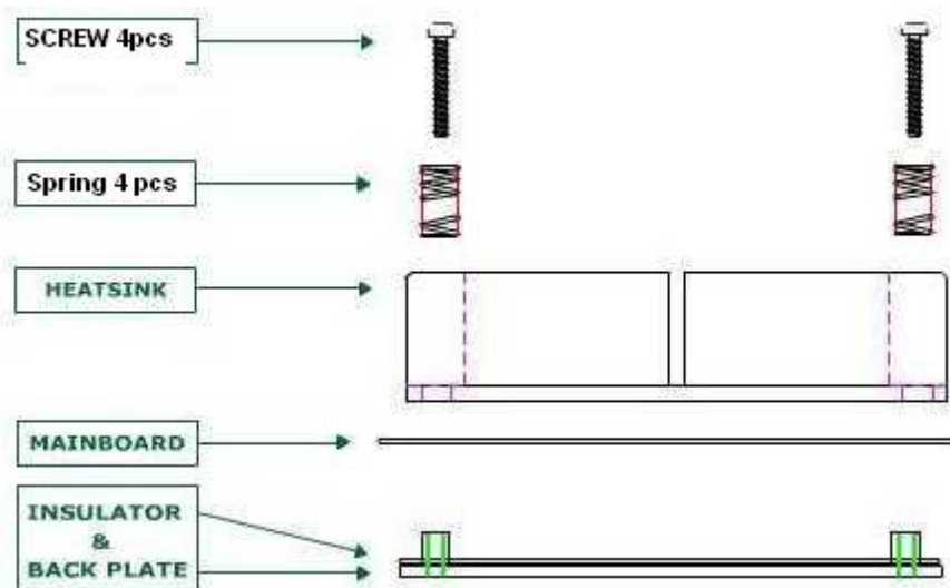
Figure 6: CPU Heatsink
