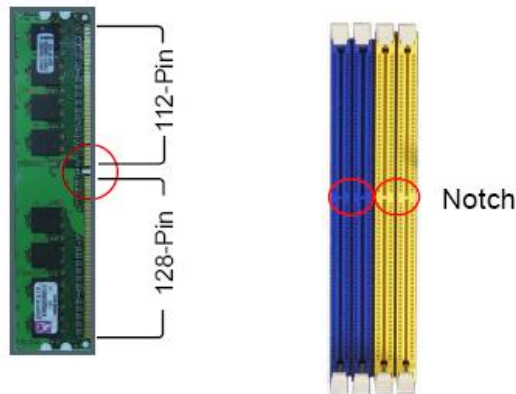
Figure 4: Memory Sockets
