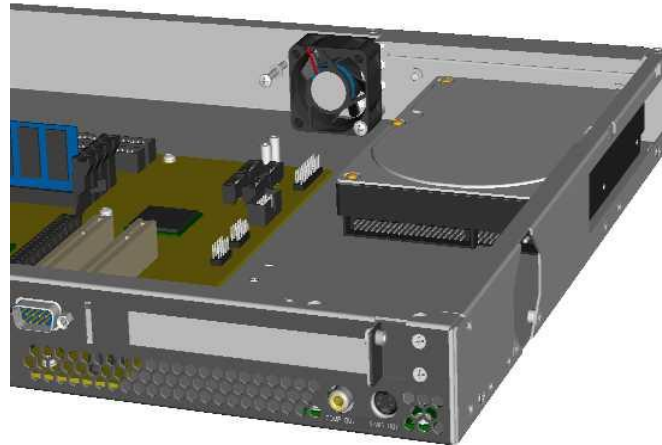
Figure 9: Chassis Fan Assembly
