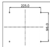
Wall Mounting Hole Dim.
