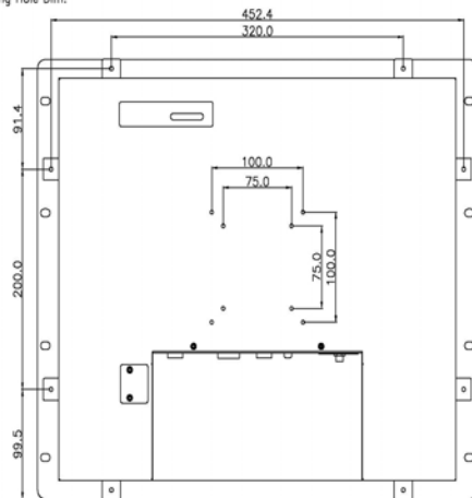
Wall Mounting Hole Dim.
